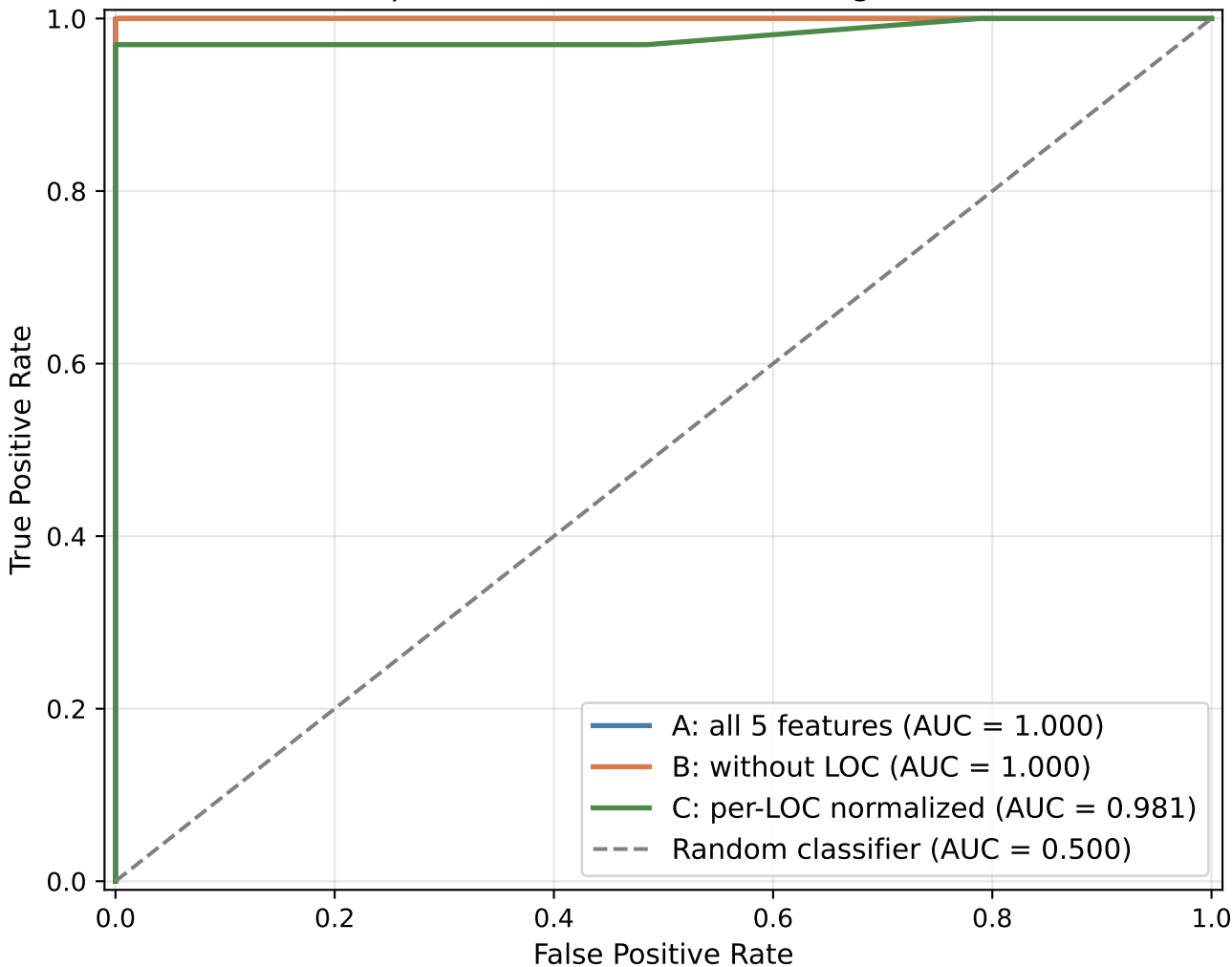
Figure 3: ROC curves for AI vs Human classification (comparison across feature configurations)
